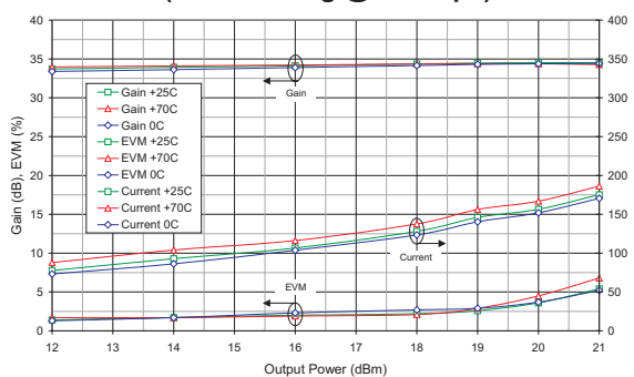
Figure 6: Gain, Current, EVM vs. Output Power at 2.462 GHz, 3.3 V (IEEE 802.11g @ 54 Mbps)
